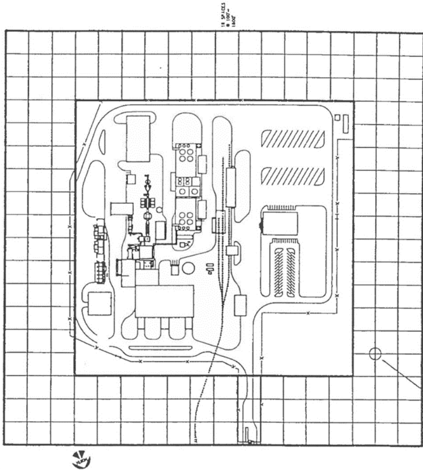
15 SPACES = 100'-0" FIGURE 1-C-3 SOILS SAMPLING GRID EXTERNAL TO THE FACILITY PROPER (TYP) (REFER TO APPENDIX L.C. SECTION J.4) CLIVE INCINERATION FACILITY EACH GRID NODE WILL BE SEQUENTIALLY NUMBERED
